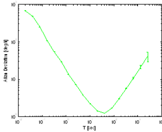
Fig. 8. AD plot for Y-Gyro with percentage errors (I bar)
