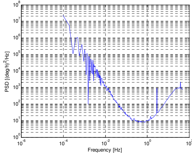
Fig. 6. X-Gyro PSD after frequency averaging
